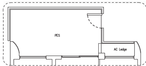
TYPE B3-Pb 81 sq m | 872 sq ft (including PES of 21 sq m/ 226 sq ft) #01-19 #01-26 #01-33
