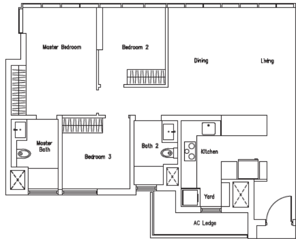
TYPE C3 92 sq m | 990 sq ft #02-20 TO #16-20 #02-27 TO #16-27
