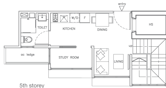
5th storey
