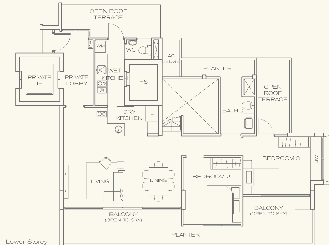
Lower Storey
