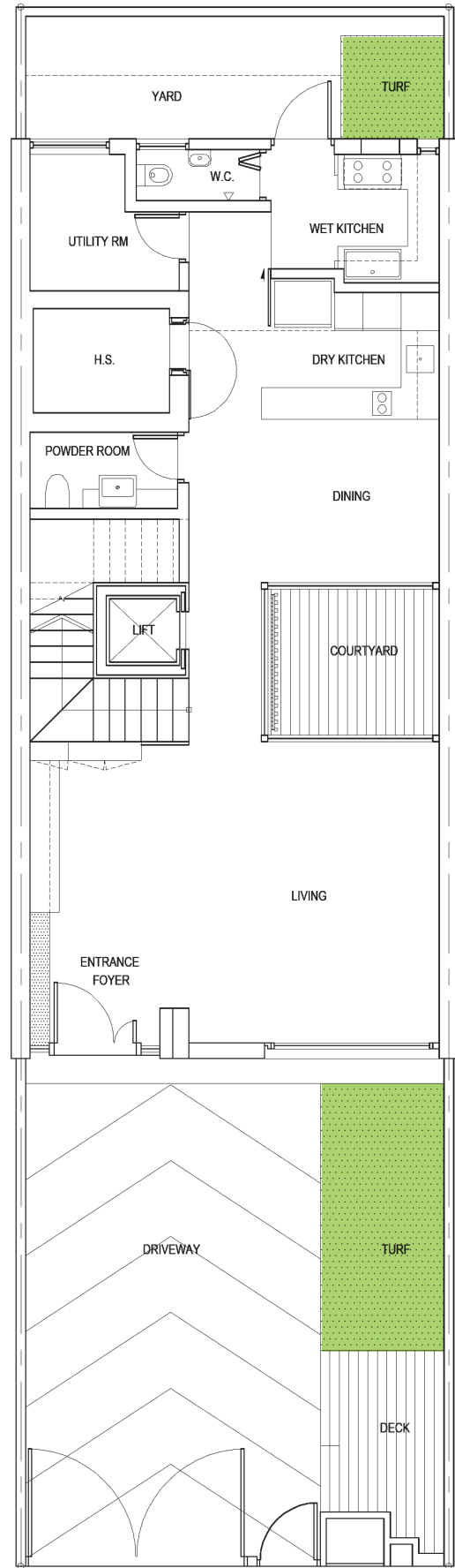
1ST STOREY PLAN
