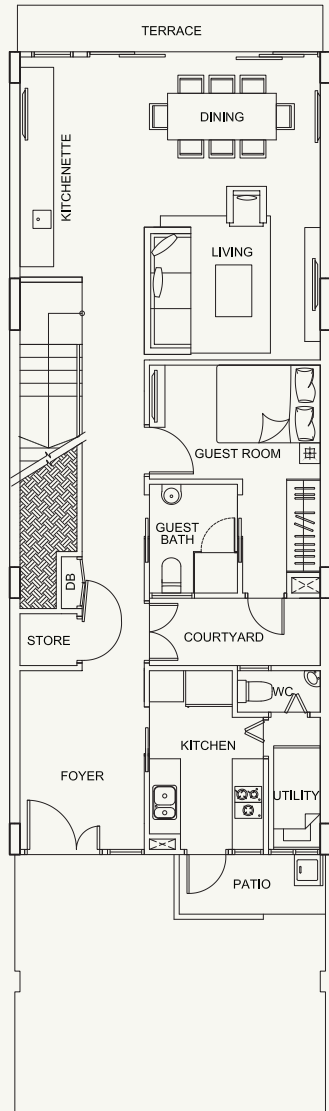
1st Storey
