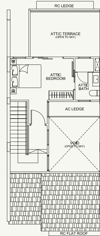
Attic
