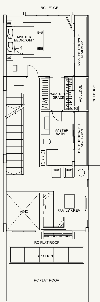
2nd Storey
