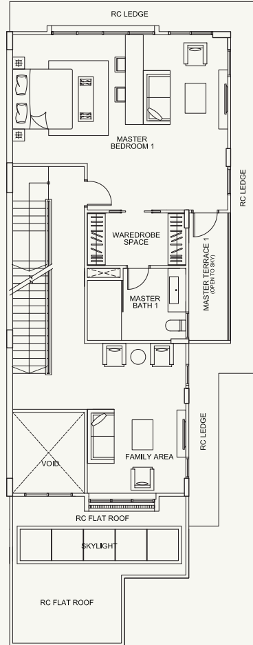
2nd Storey
