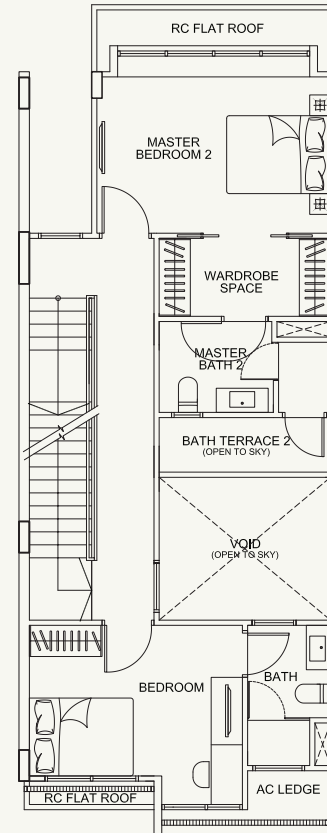
3rd Storey
