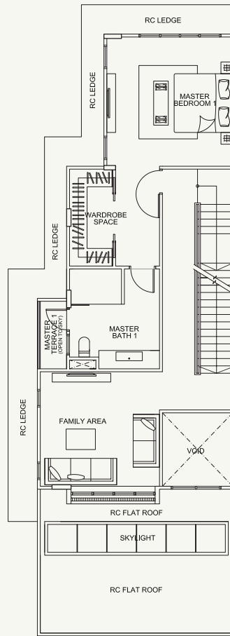
2nd Storey
