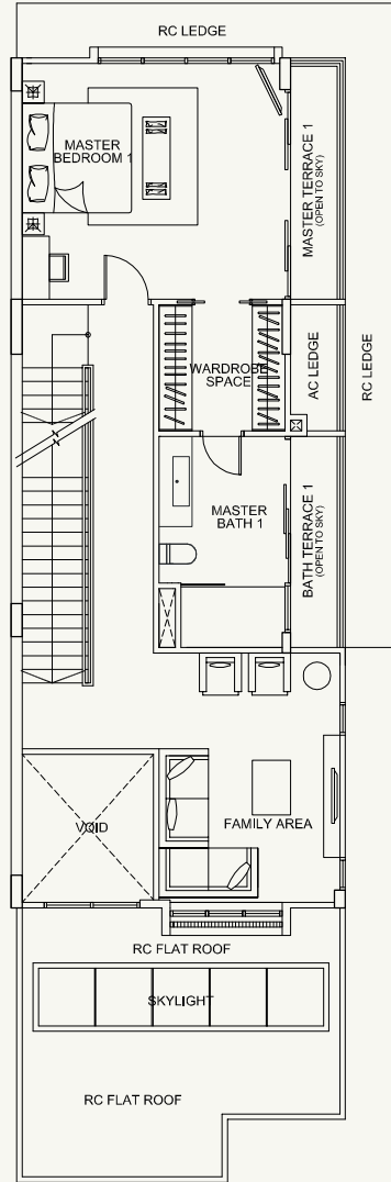
2nd Storey
