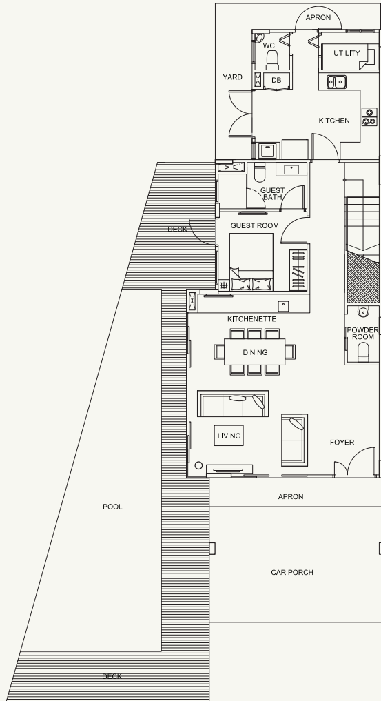
1st Storey
