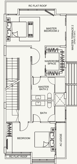
3rd Storey
