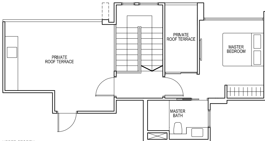
UPPER STOREY
