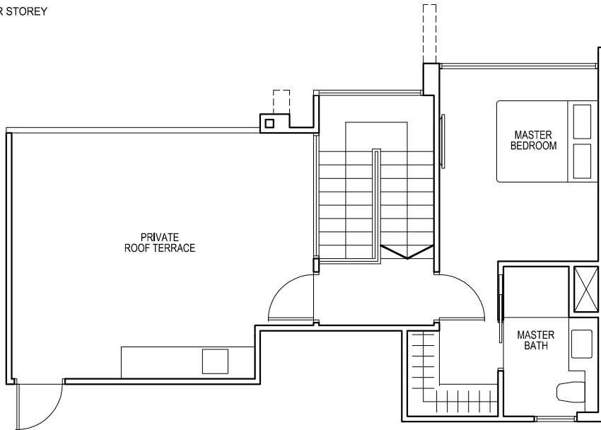
UPPER STOREY
